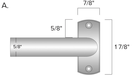
48" SPAN BETWEEN BRACKETS STANDARD RETURN - 2 1/2" MINIMUM RETURN - 2"
